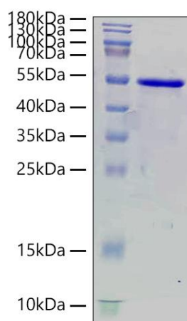
Figure 1. SDS-PAGE
